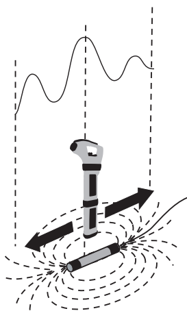
Forward/Back Locate
