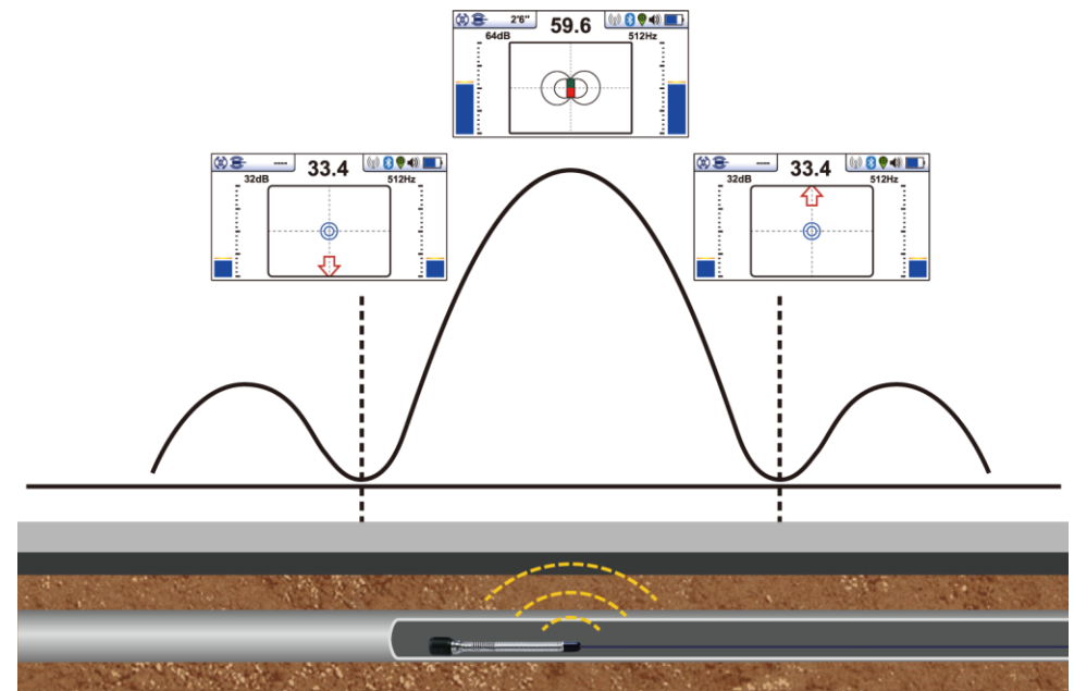
Receiver display
