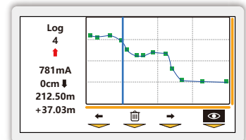
Review Screen - to review points of the complete graph. Shows LF current, total survey distance, distance from the previous measurement.
